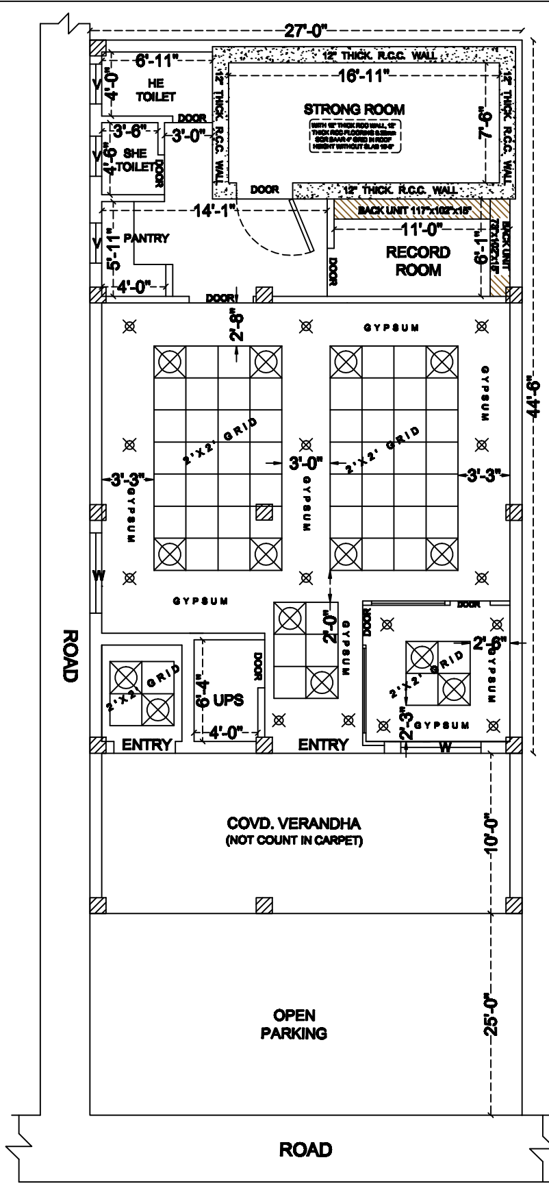
PROPOSED BUILDING PLAN
