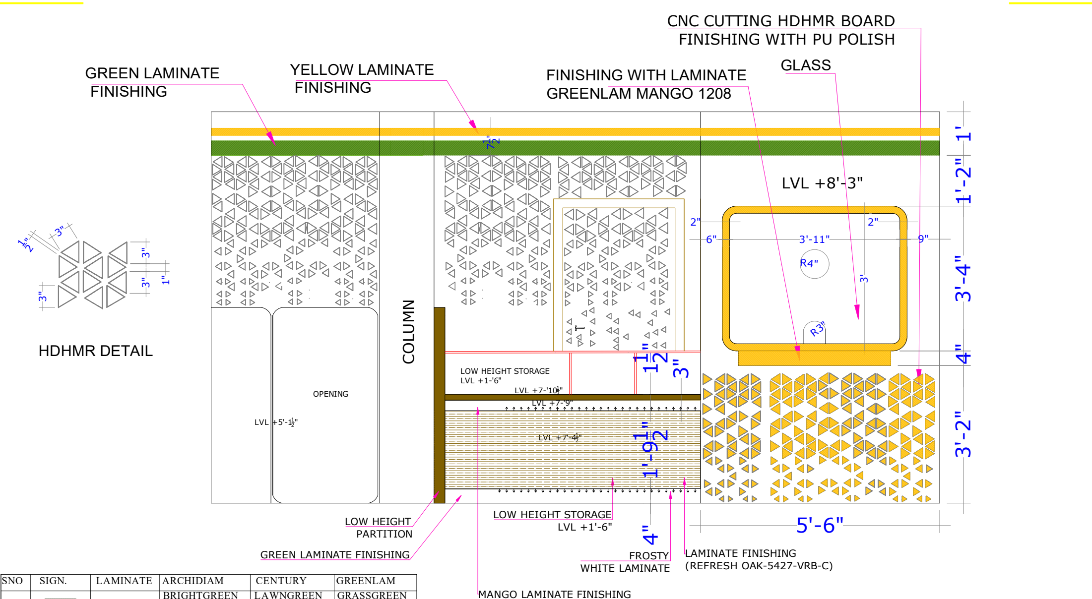
(A3) WALL ELEVATION
