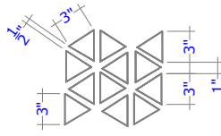
HDHMR DETAIL
