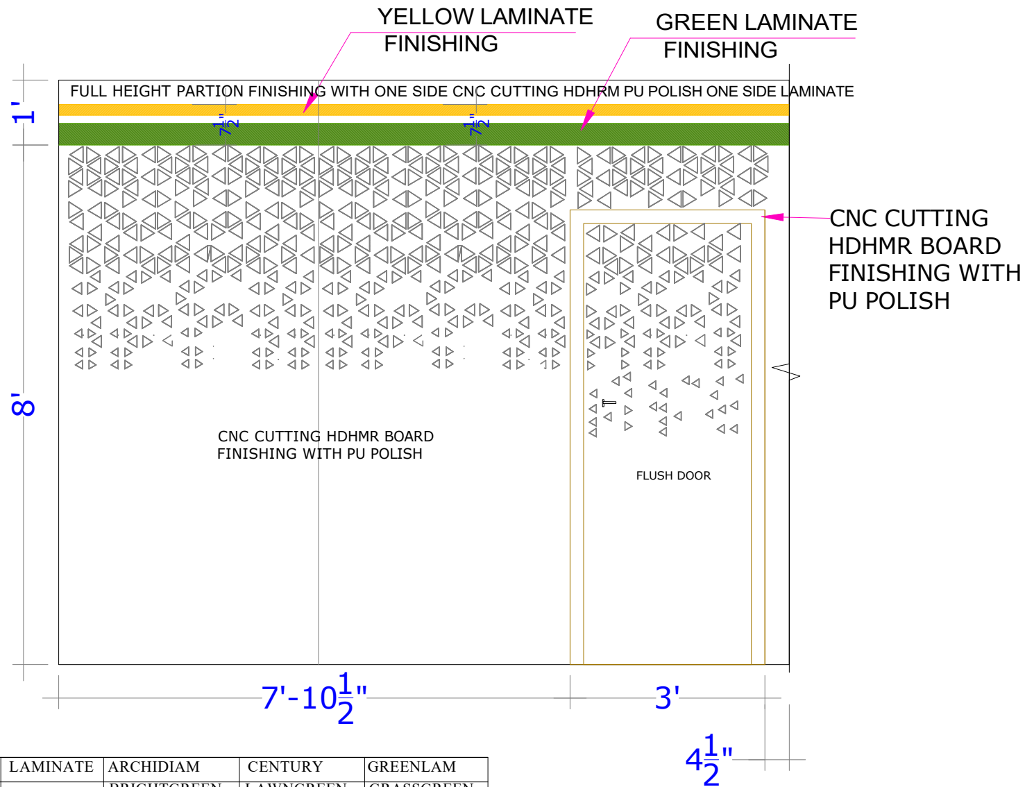
HDHMR DETAIL
