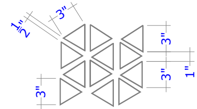
HDHMR DETAIL
